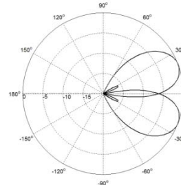
Azimuth(1710-2690MHz)
