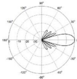
Elevation(698-960MHz)
