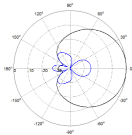
Azimuth(698-960MHz)
